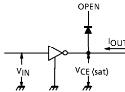
2. V_{CE(sat)}
